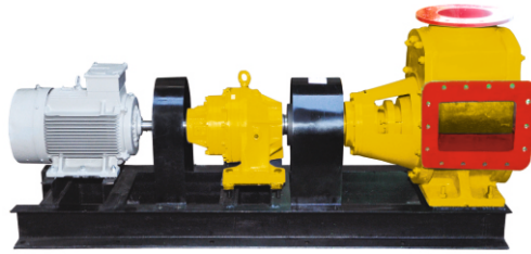
MASSECUITE PUMPS
